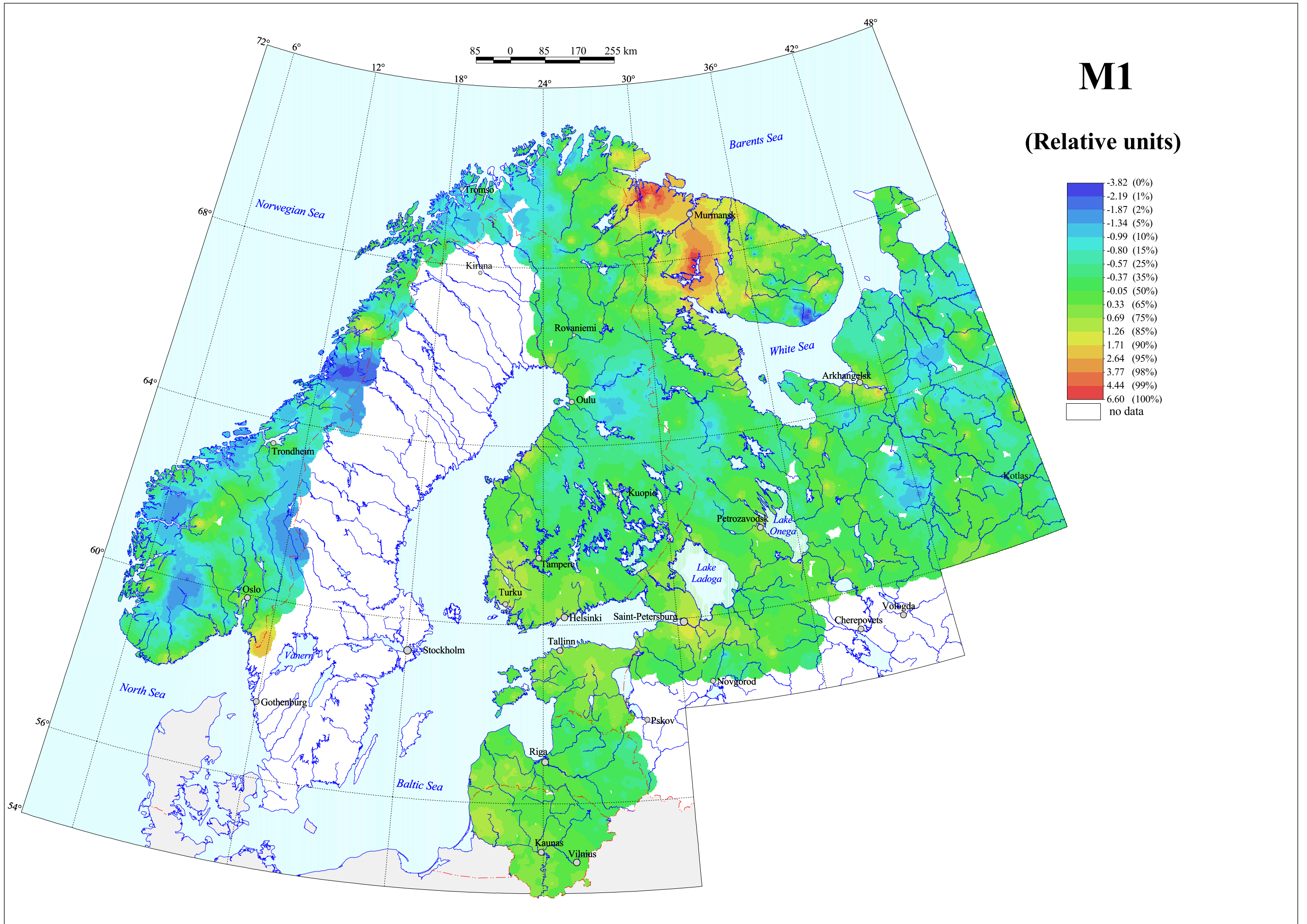
M1 (Co, Cr, Cu, Ni) in Terrestrial Moss, Total Content
